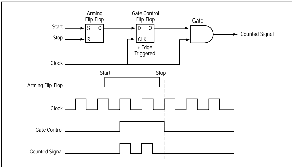
Figure 27. Synchronized Gating
